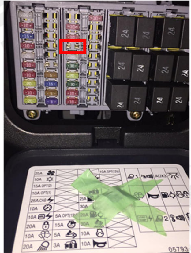
TB2150 Uninstall Fuse Example Cover Open
