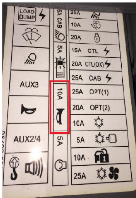
TB290 Fuse Detail
