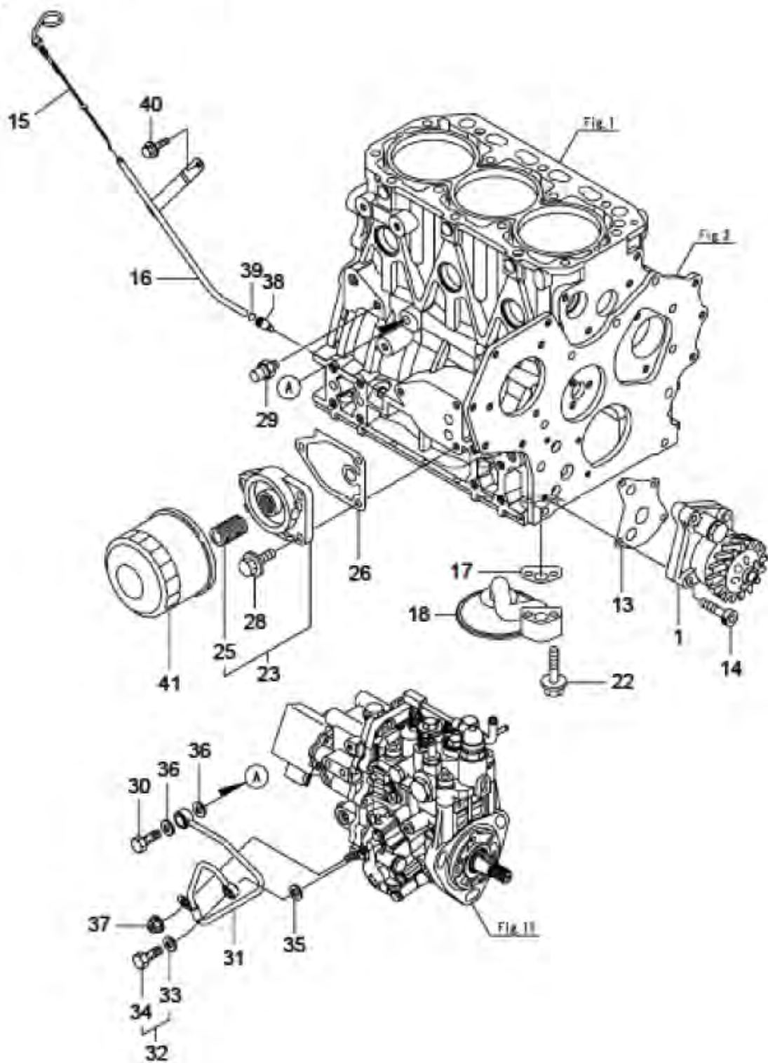
Fig.9. LUB. OIL SYSTEM
