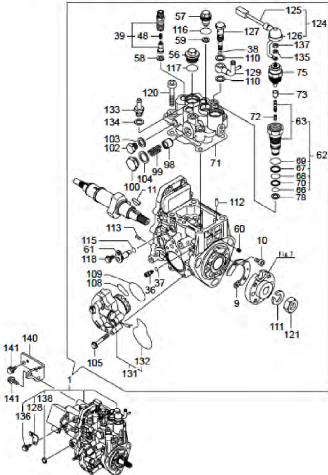
Fig.11. FUEL INJECTION PUMP
