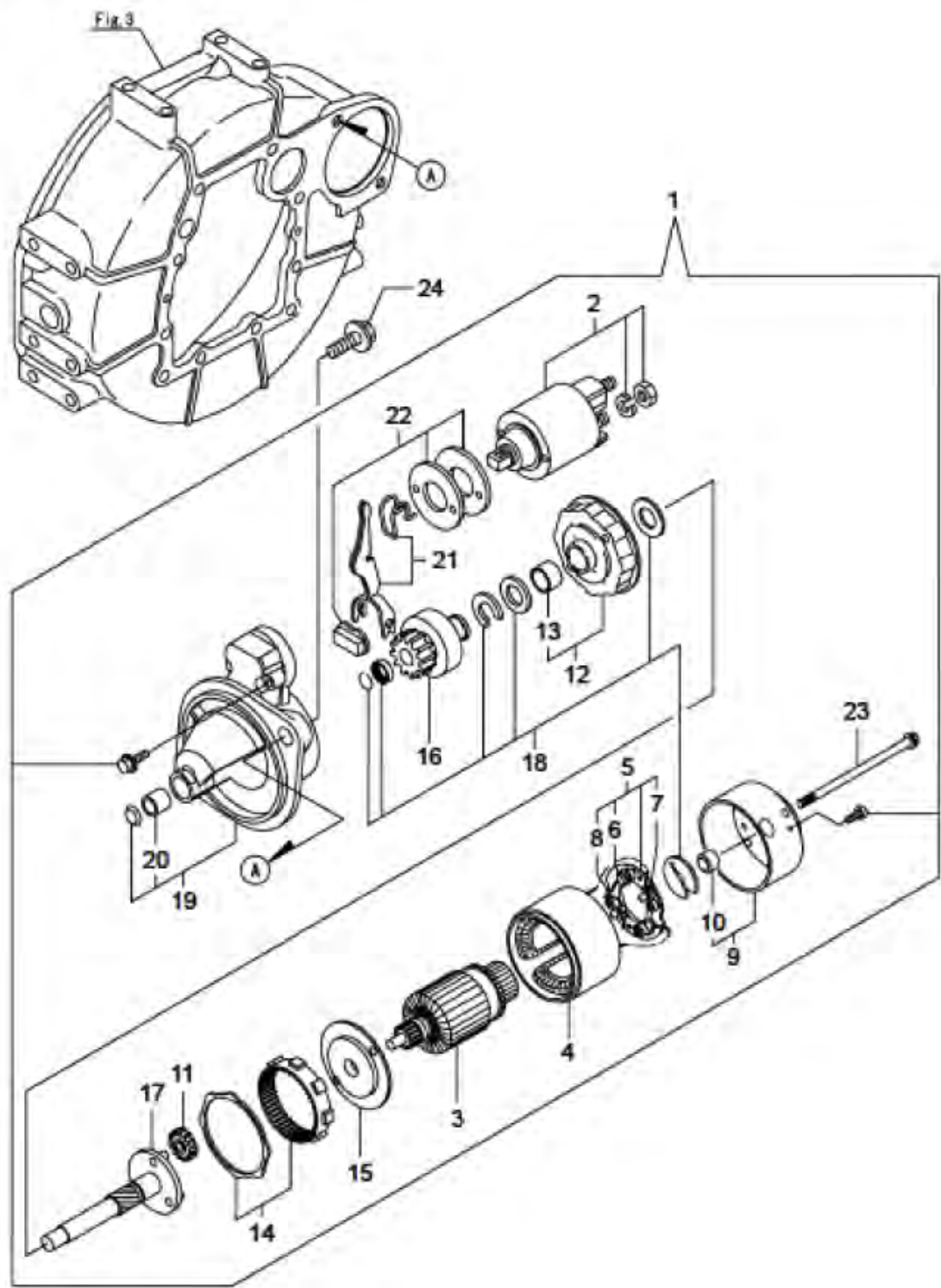
DCD50-M03400 ENGINE Fig.15. STARTER MOTOR
