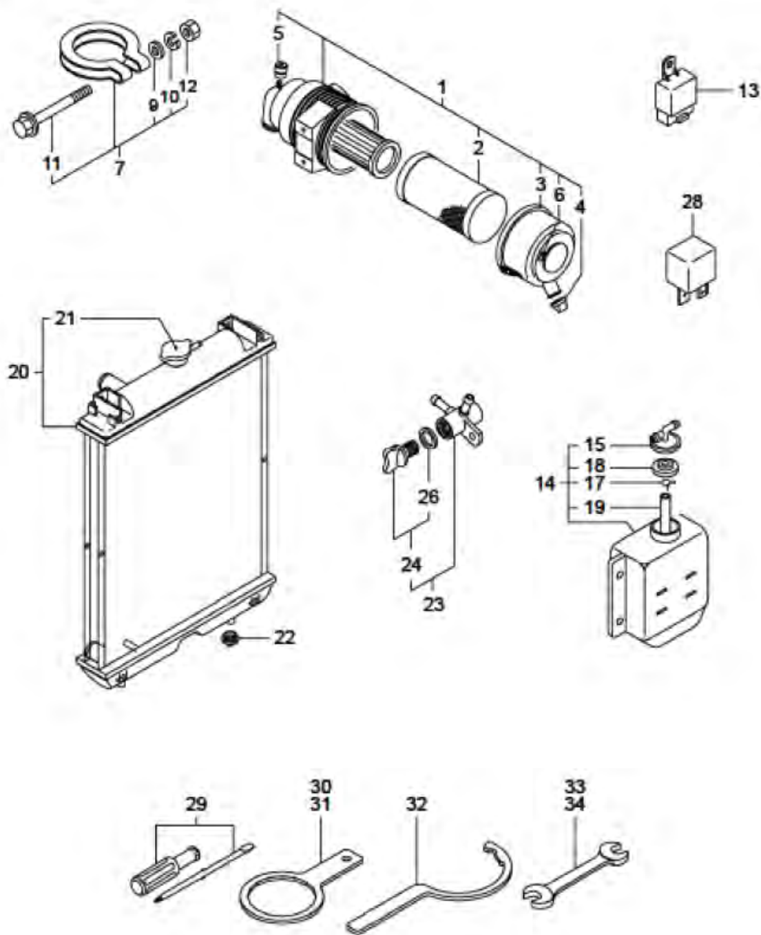
DCD50-M03400 ENGINE Fig.18. ACCESSORY
