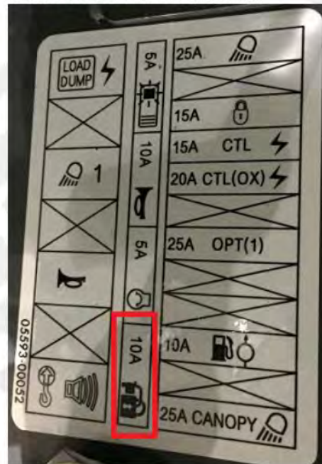
TB230 TB240 TB260 Fuse Detail
