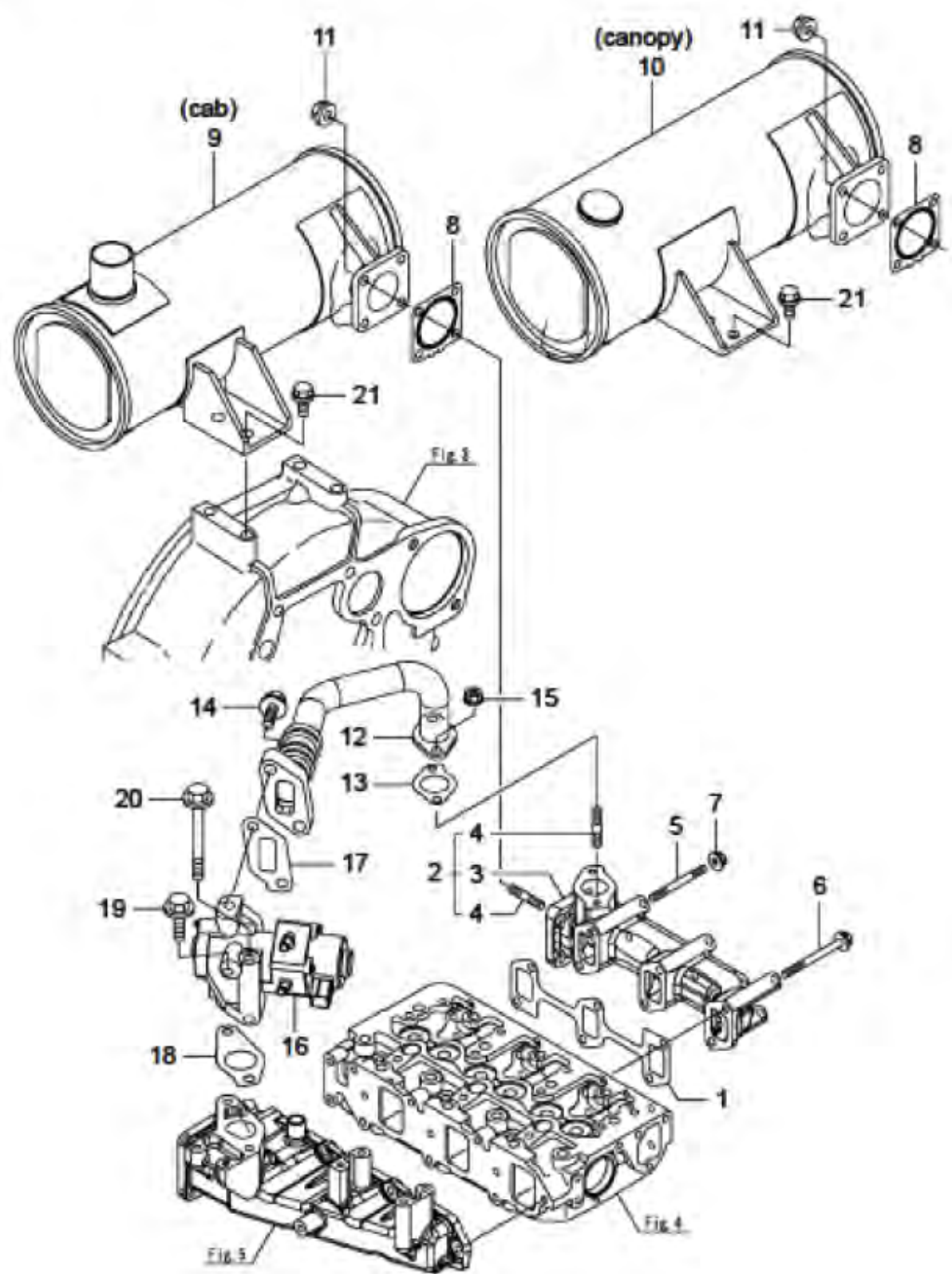
Fig.6. EXHAUST MANIFOLD & SILENCER
