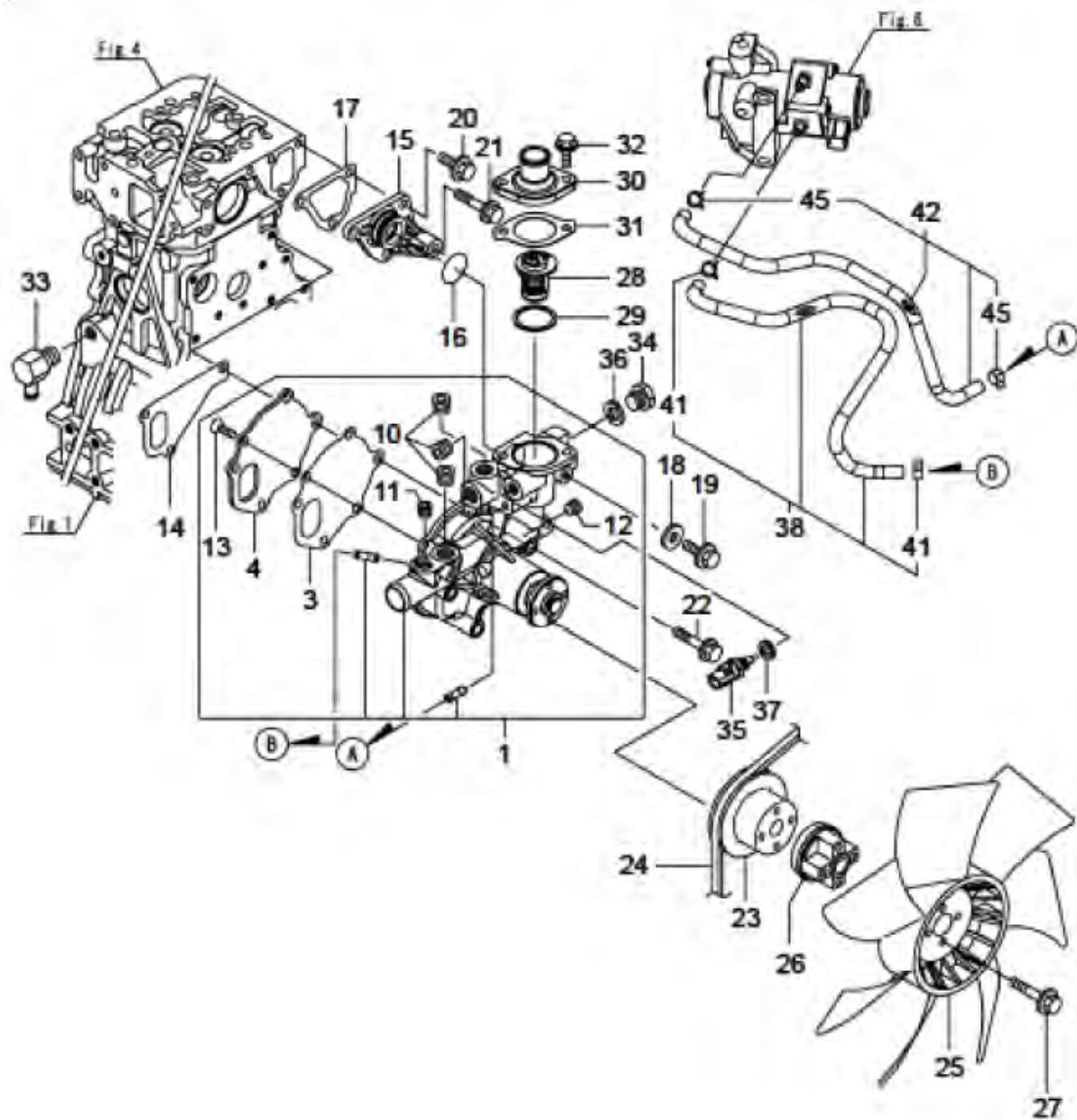
Fig.10. COOLING WATER SYSTEM
