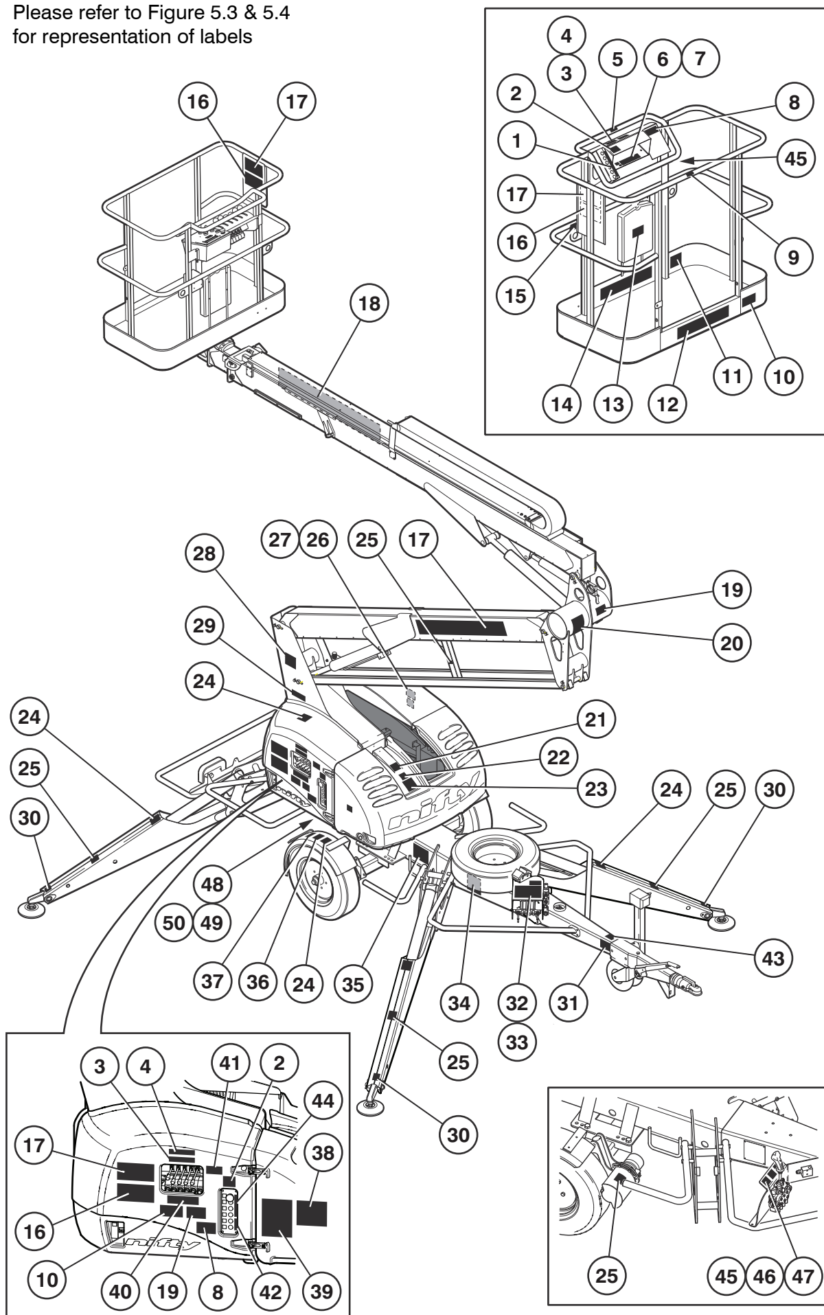
Figure 5.1 Label locations 150T
