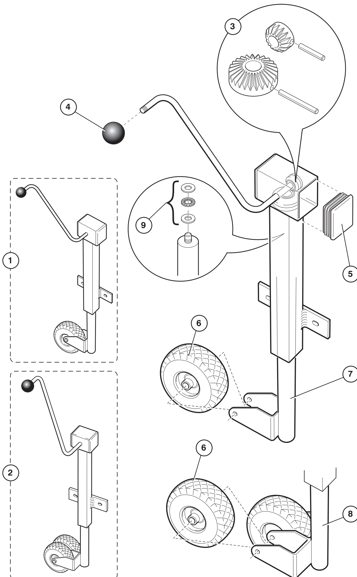
Figure 1.6 Jockey wheel assembly
