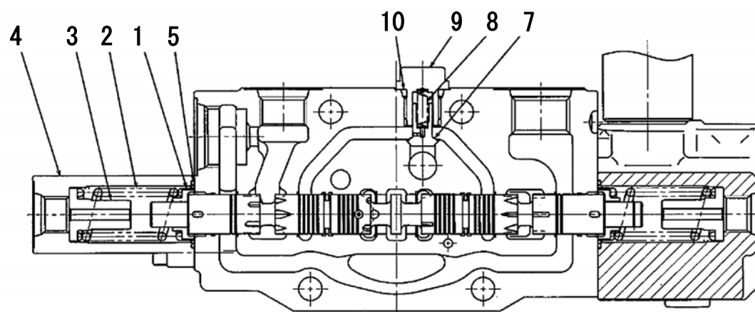
SECTION "X-X"
