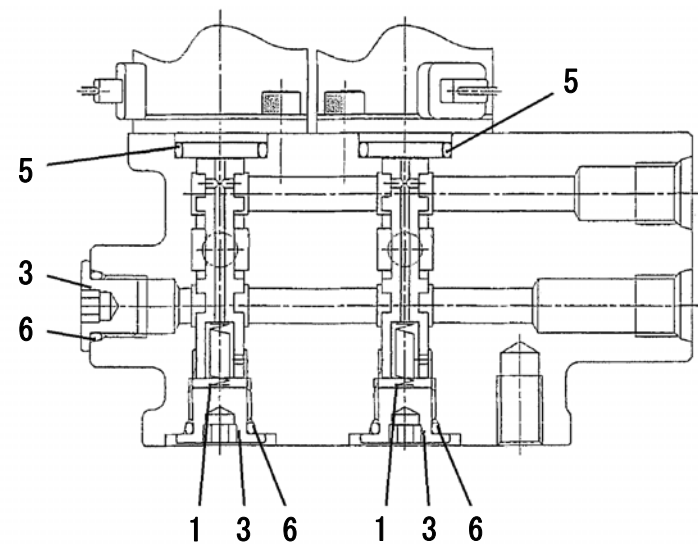
SECTION "X-X"
