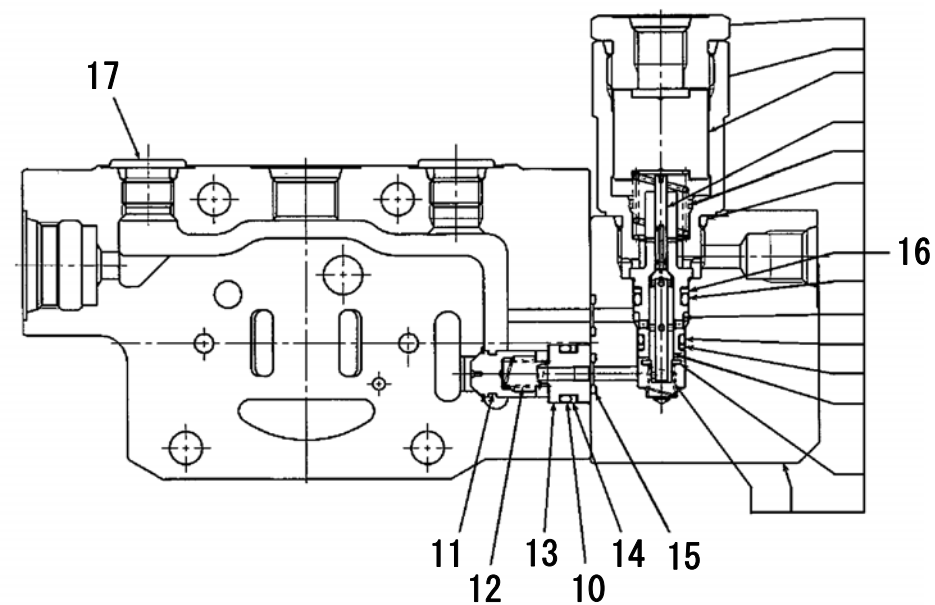
SECTION "Y-Y"
