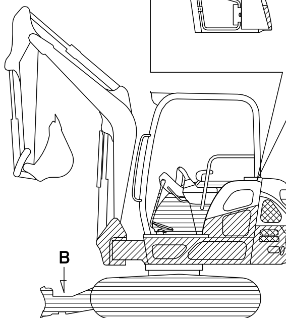
VIEW "B" angle blade type
