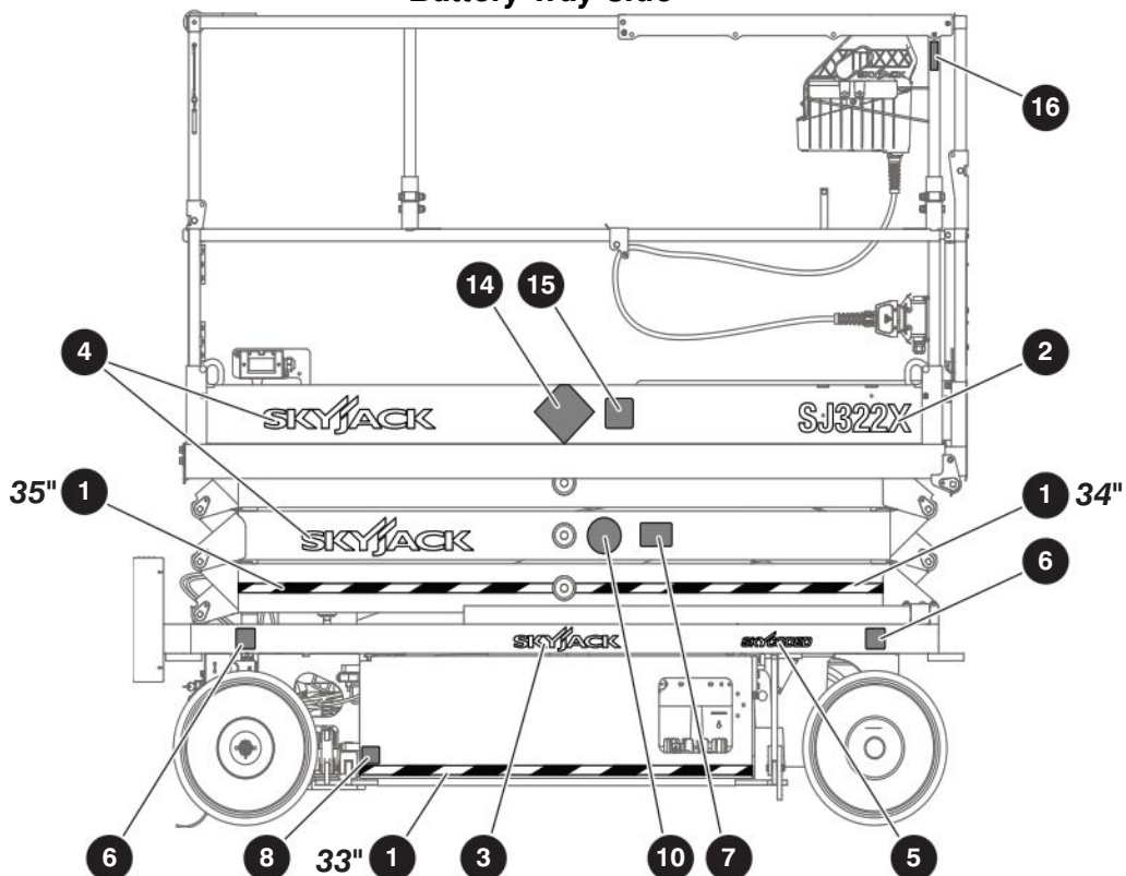
Battery Tray Side
