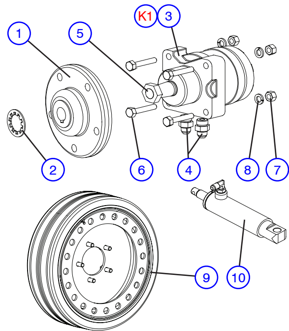
Pin Brake (Models 32xx)
