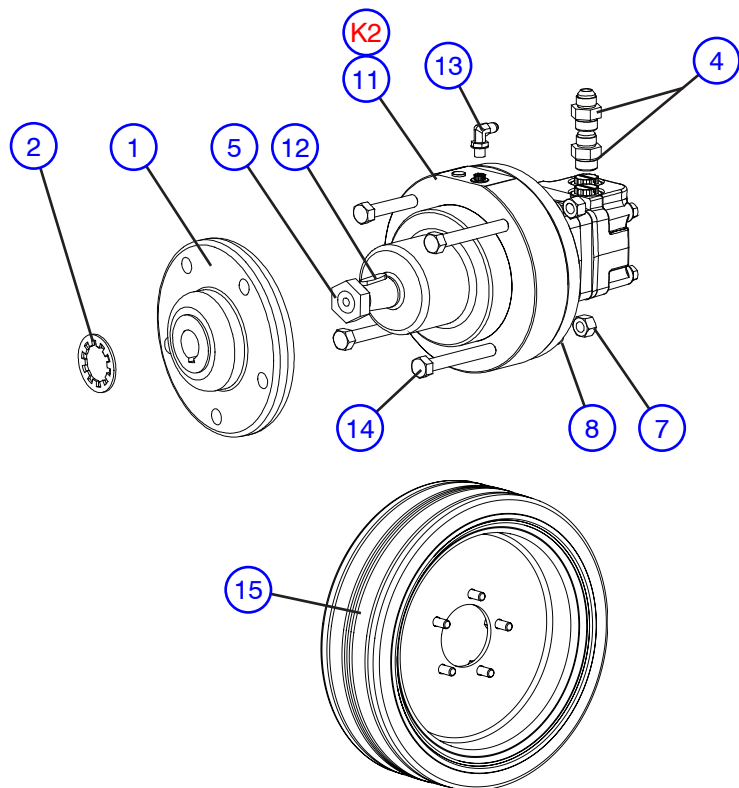
Disc Brake (Models 46xx)
