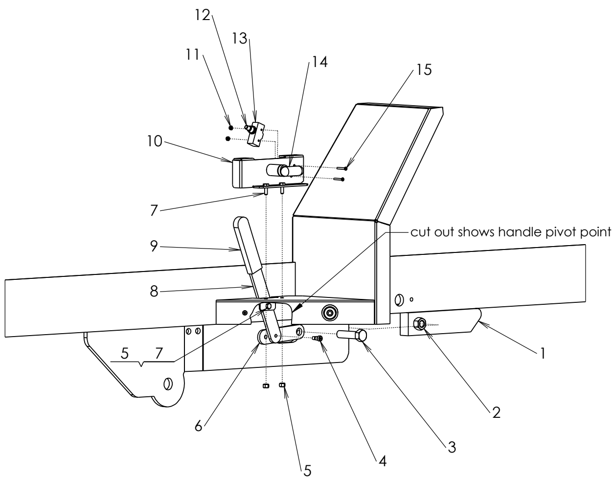
AXLE LOCK ASSEMBLY FOR MODEL U12 -ALSO MODEL U14 PRIOR TO 2/2016 -ALSO MODEL U16 PRIOR TO 2/2016
