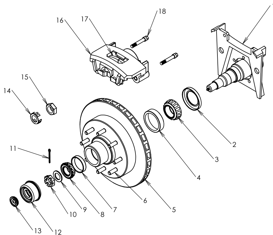
DISC BRAKE REPAIR PARTS
