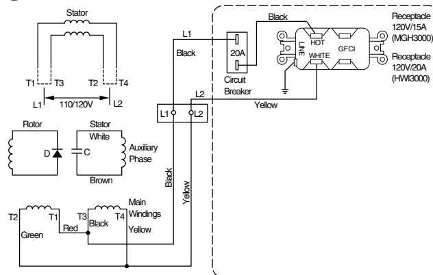
Figure 26 - Wiring Diagram, Models HWI3000, MGH3000, and MGH3000PR
