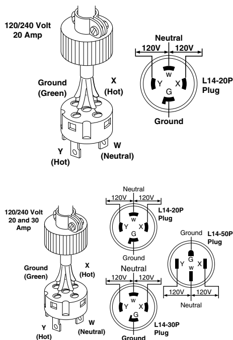
Figure 16 - Cord and Plug Configurations
