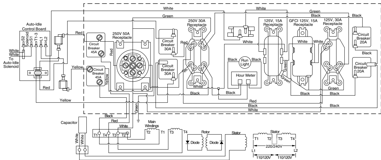
Figure 29 - Wiring Diagram, Model MGH10000
