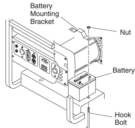
Figure 10 - Battery Hold-Down System (Model MGH7000C Shown)
