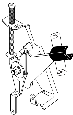
Figure 20 - Engine Lever In ON Position (Model MGH3000PR Only)
