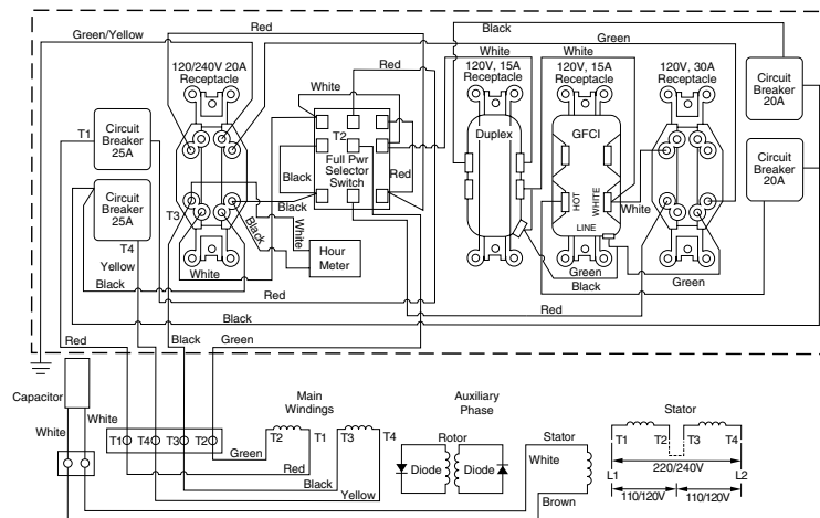
Figure 27 - Wiring Diagram, Models MGH4000C, MGH5000C, MGH5000CIE, and MGH6000C
