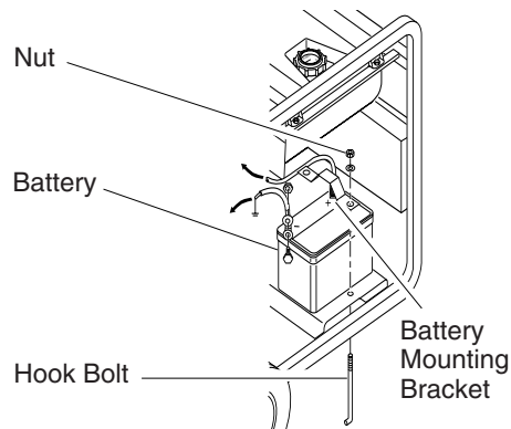
Figure 11 - Battery Hold-Down System (Model MGH10000 Shown)
