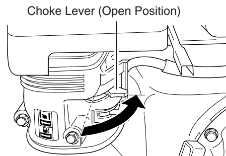
Figure 23 - Choke Lever Opened (Model MGH7000C Shown)
