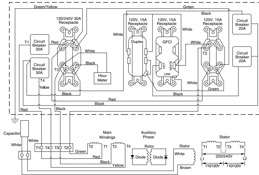
Figure 28 - Wiring Diagram, Model MGH7000C
