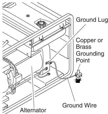
Figure 14 - Grounding Generator (Model MGH4000C Shown)
