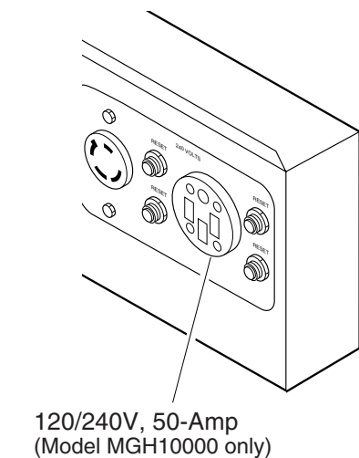
Figure 15 - Receptacle Locations
