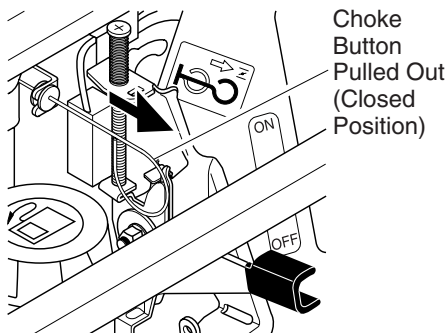
Figure 18 - Choke Rod Closed (Model MGH3000PR Only)
