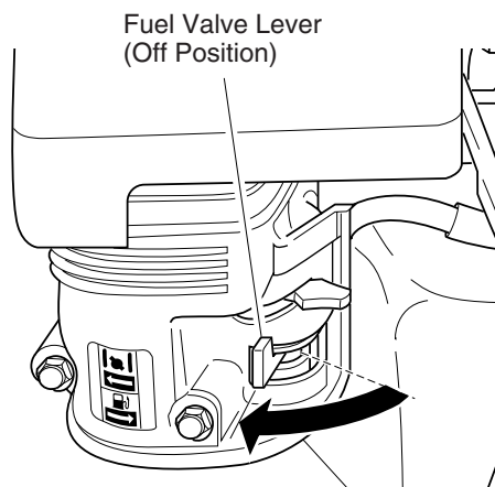
Figure 25 - Fuel Valve Lever Off (Model MGH7000C Shown)
