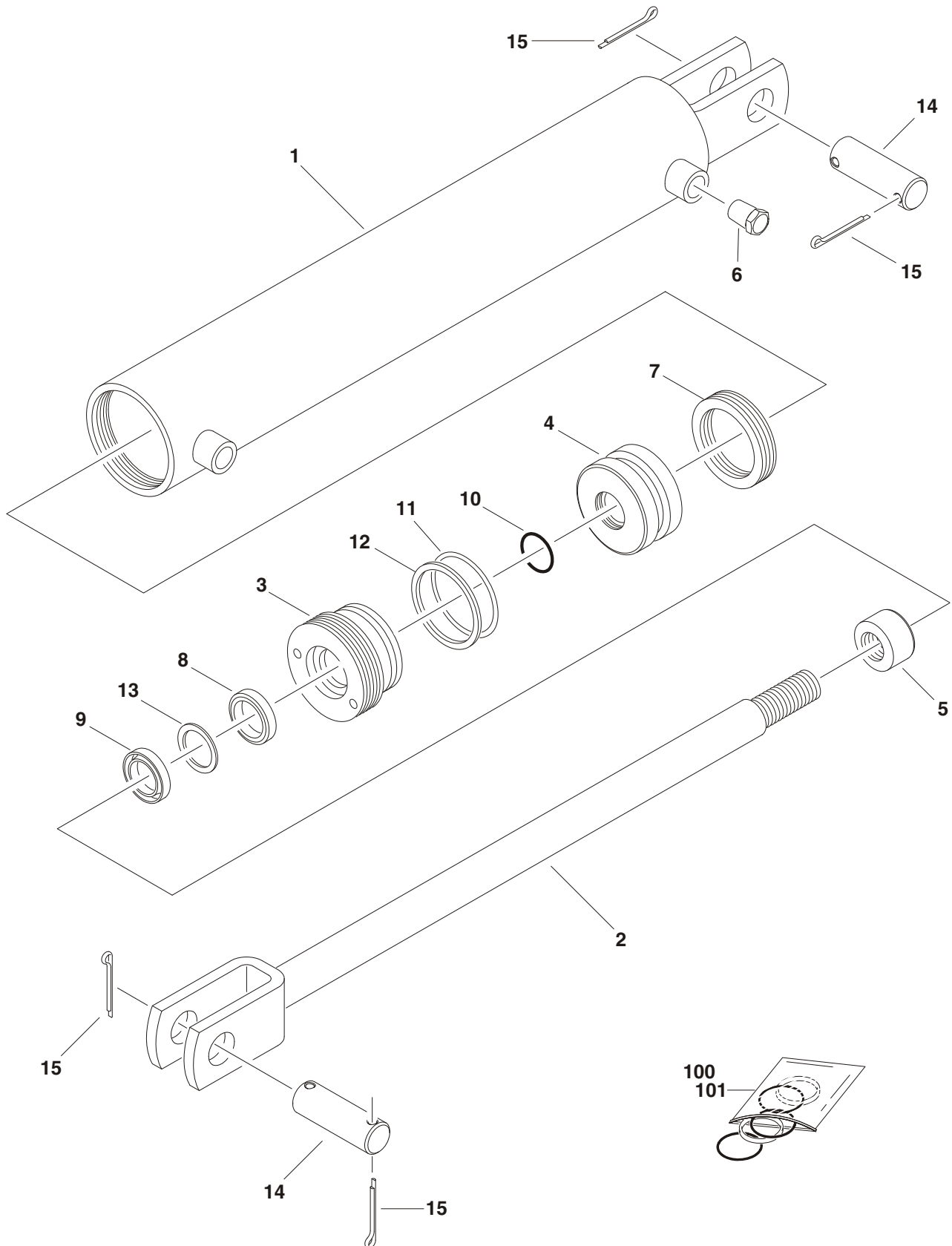
FIGURE 1-7. CYLINDER ASSEMBLY (ORIGINAL EQUIPMENT)
