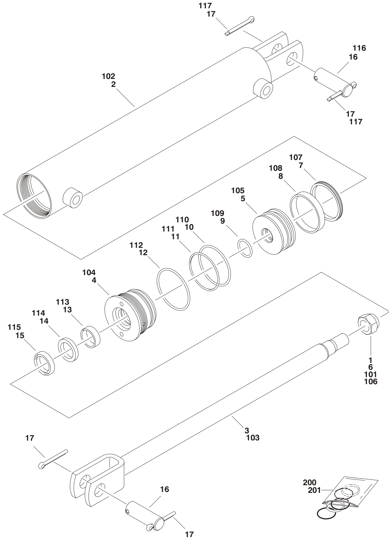
FIGURE 1-8. CYLINDER ASSEMBLY (SERVICE REPLACEMENT)
