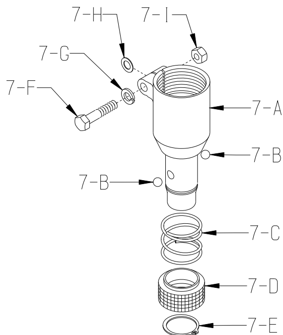
ITEM # 7 PART # C10514 CHISEL HOLDER ASSEMBLY
