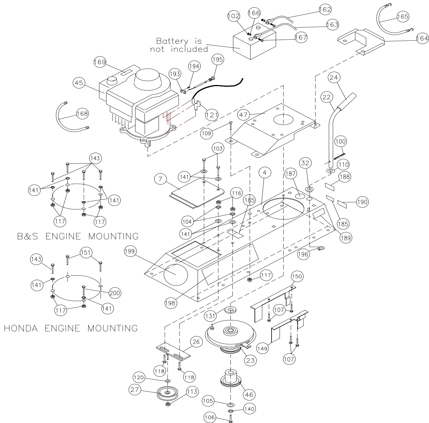
Engine and Engine Base Assembly Figure 6
